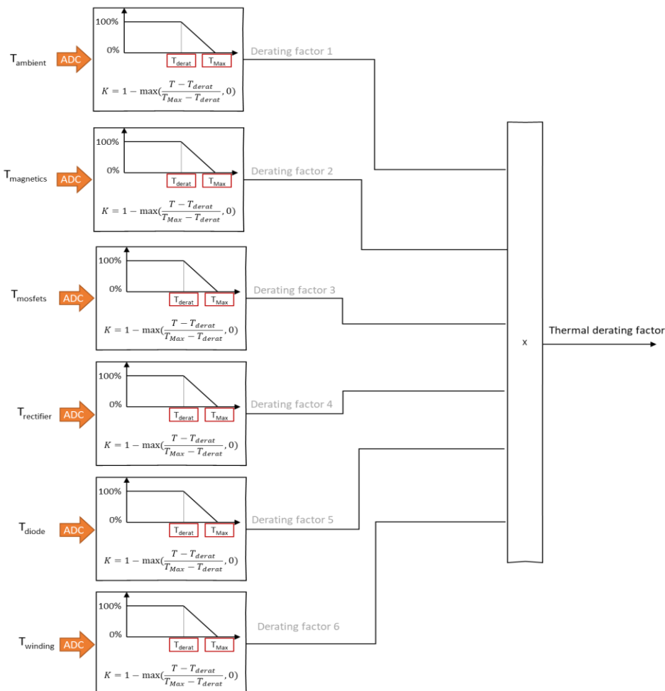
Figure 21: Thermal derating
