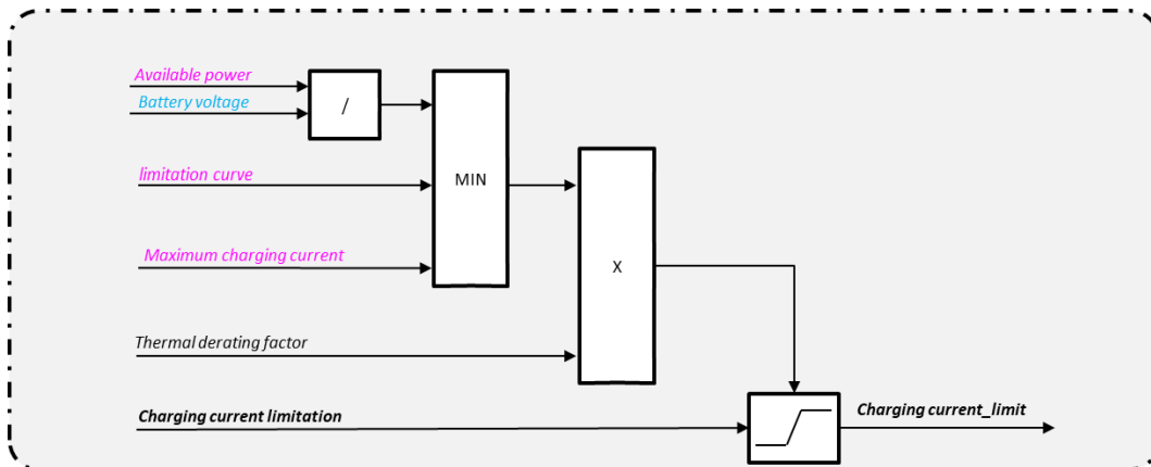
Figure 19: DC Charging current limitation
