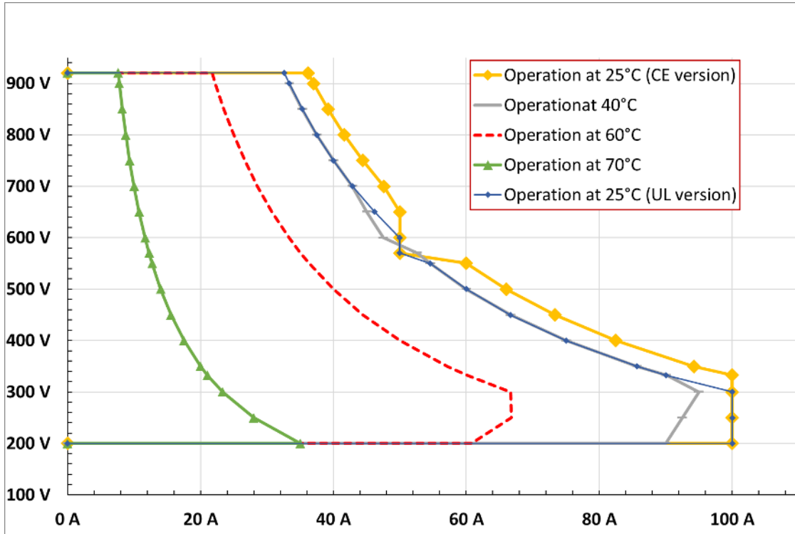
Figure 5: detailed safe operating area in function of the ambient temperature for HW V1.1.0 and forward
